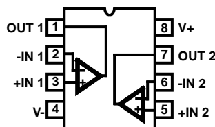
HA-5222 (CERDIP) TOP VIEW
