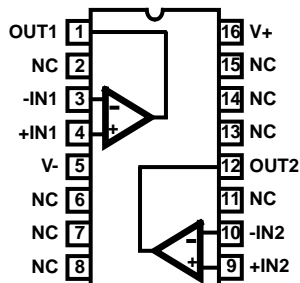
HA-5222 (PDIP, SOIC) TOP VIEW
